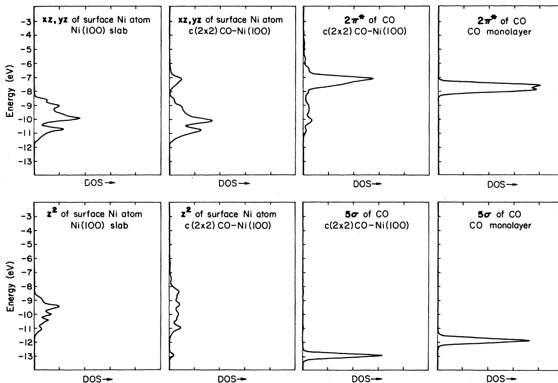
FIG. 6. "Interaction diagrams" for 5\sigma and 2\pi^* of c(2\times 2)\text{CO-Ni}(100) . The extreme left and right panels in each case show the contributions of the appropriate orbitals ( z^2 for 5\sigma , xz, yz for 2\pi^* ) of a surface metal atom (left), and of the corresponding isolated CO monolayer MO. The middle two panels then show the contributions of the same fragment MO's to the DOS of the composite chemisorption system.
